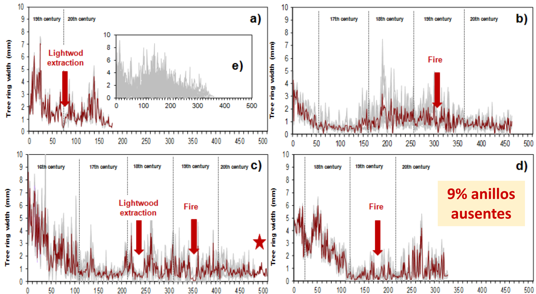
Figure 1. Tree-ring series analysed in the present paper: a) Pino Seco (SE), b) Pino de La Lajilla (LA), c) Pino de Pílancones (PI), d) Pino de Gáldar (GA), e) Inagua series. The light grey lines indicate the measurements taken in the different radii or cores (Inagua series) and the dark red ones the averages for each tree. The arrows indicate the most significant events, the star the maximum number of continuously MORs (56) and the dashed lines its approximate time range. Génova et al., 2017
